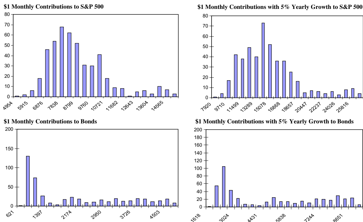
Graph 5. Distribution of 40 year S&P 500 and bond accumulations for 481 generations.
