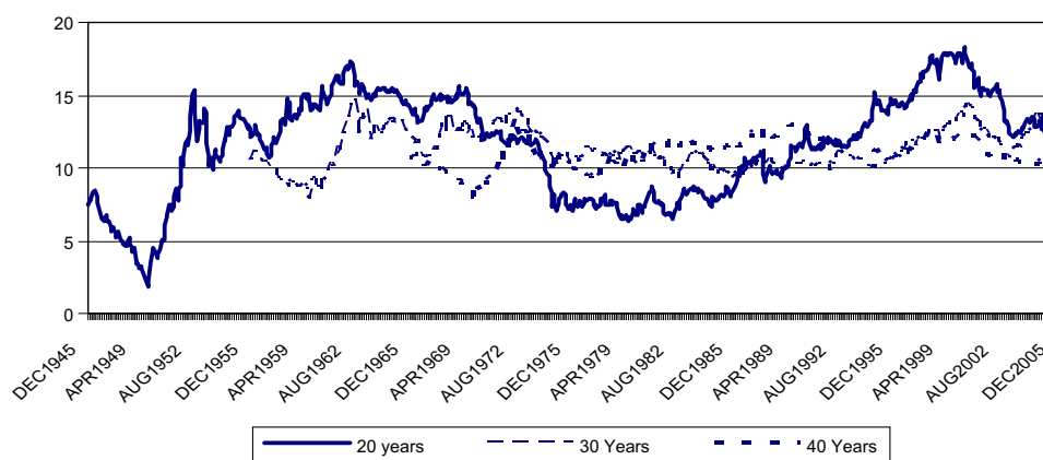
Graph 3. Time series of generational annualized means for 20–40 year investment horizons.
